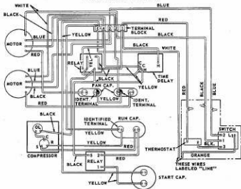
WIRING DIAGRAM No. 52712C
