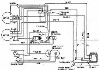
WIRING DIAGRAM No. 52712C
